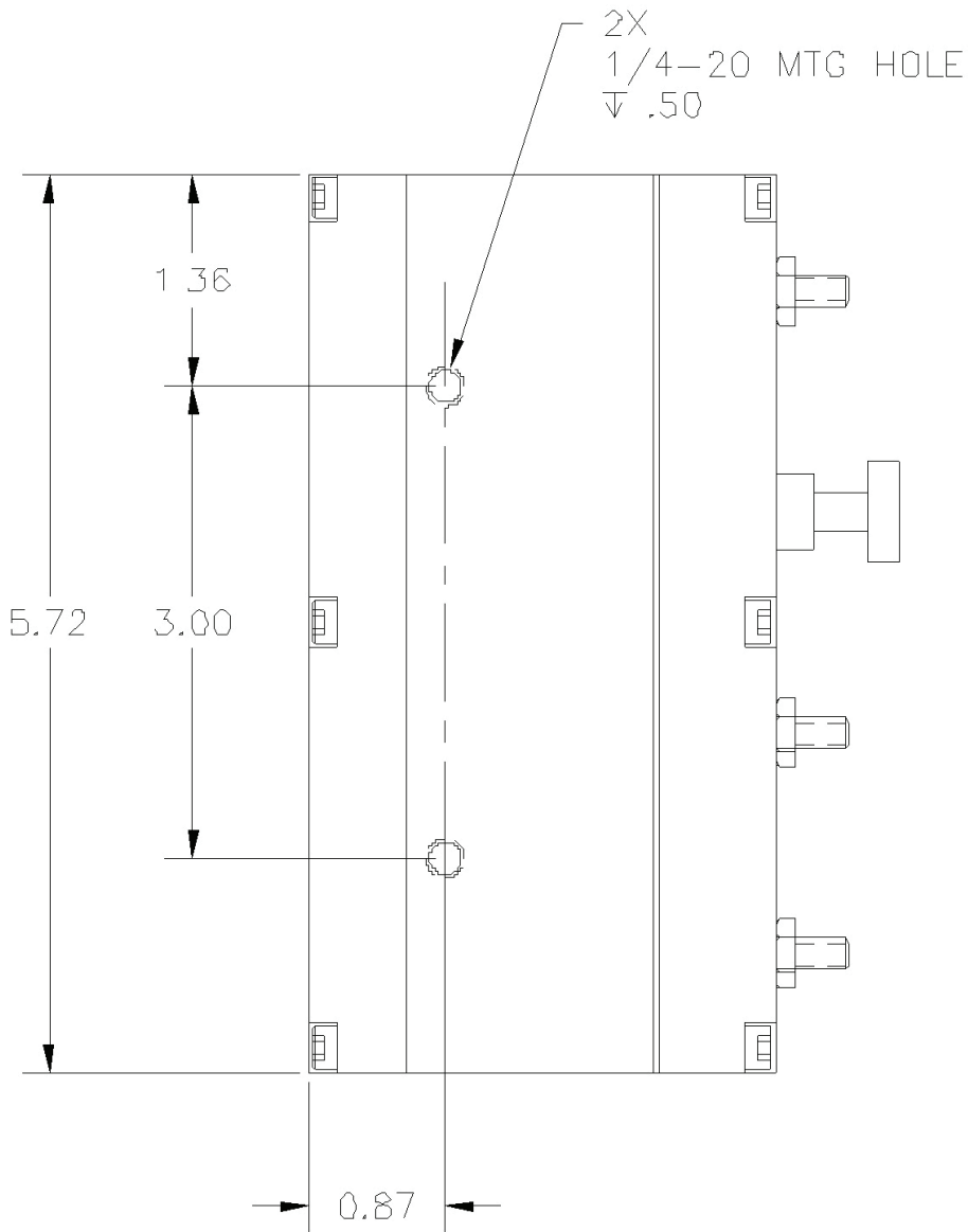
TRIDAK MODEL 340 POSITIVE-DISPLACEMENT VALVE
